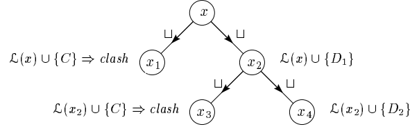
Fig. 2. Syntactic branching
