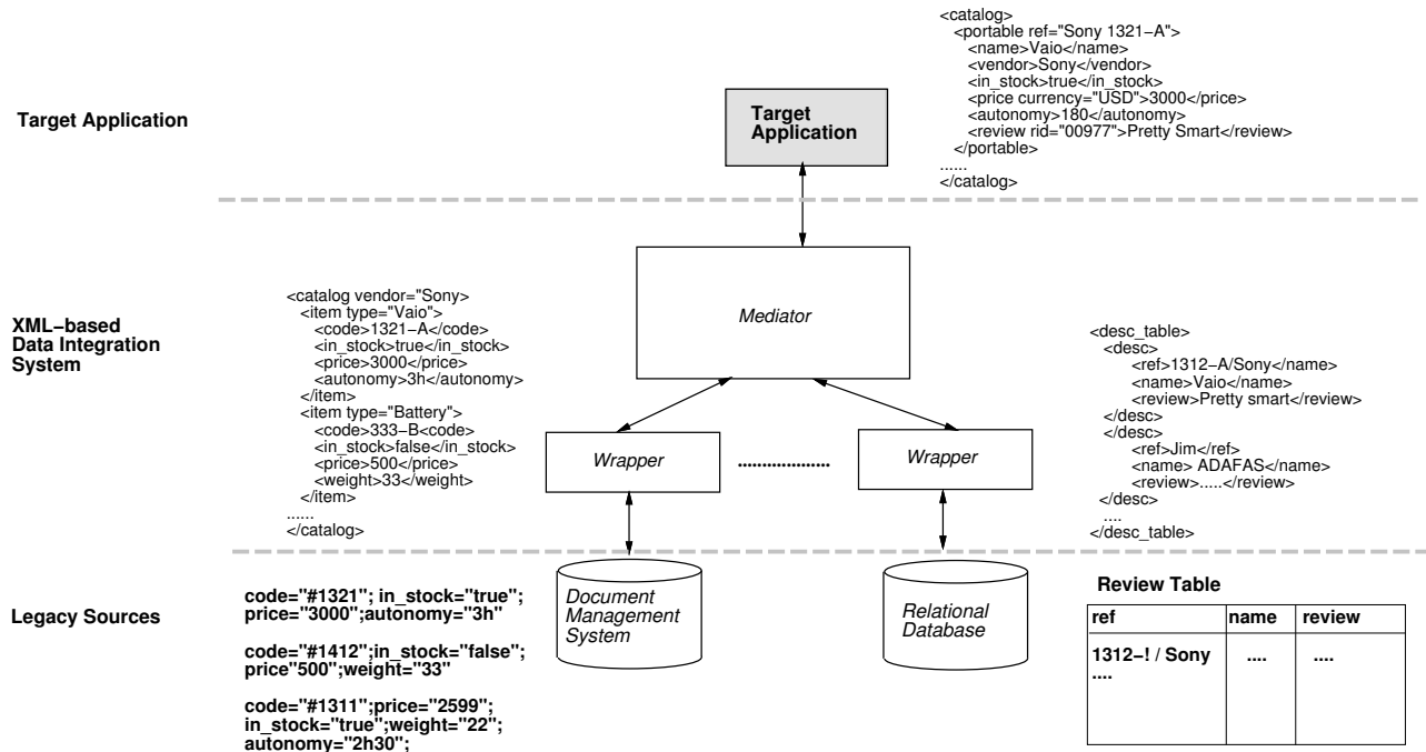
Figure 2: XML-based data integration
