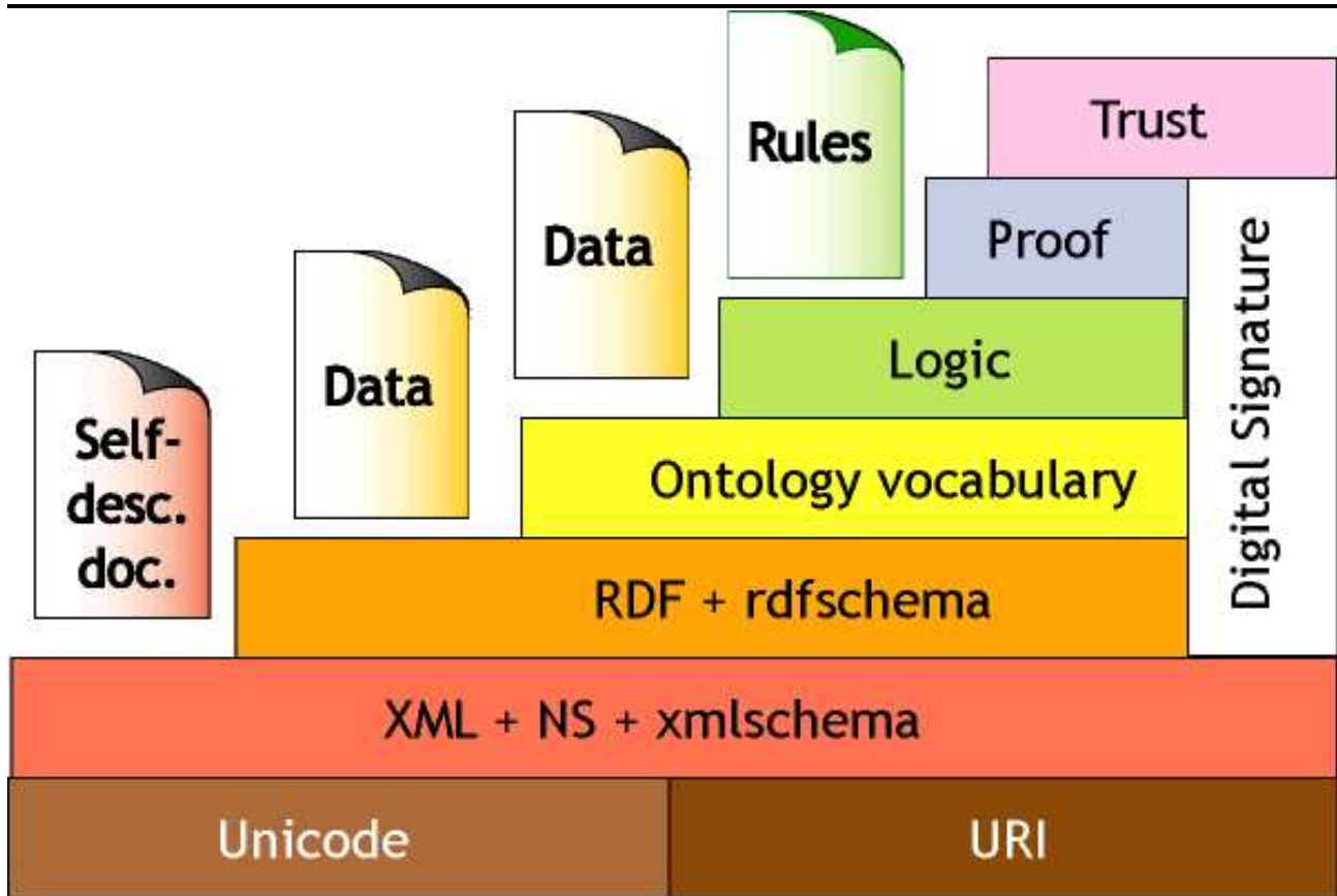
Figure 1: The Semantic Web Layer Cake
