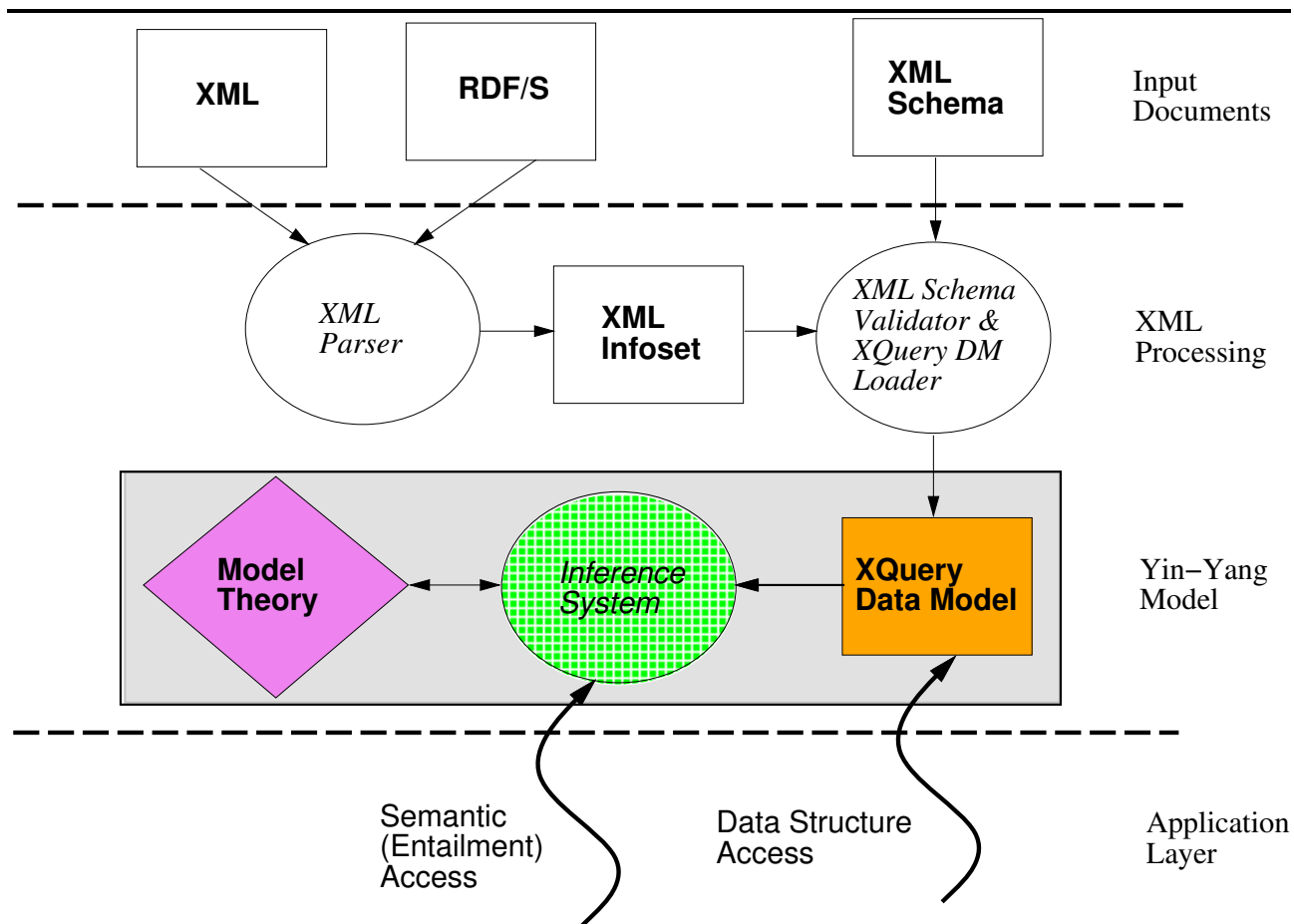
Figure 4: Yin/Yang model
