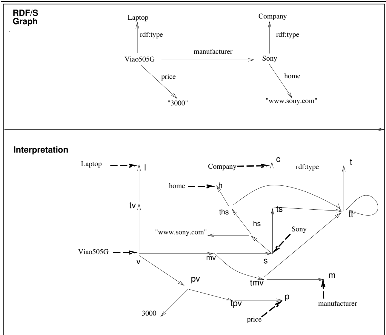
Figure 5: RDF Graph and a corresponding interpretation
